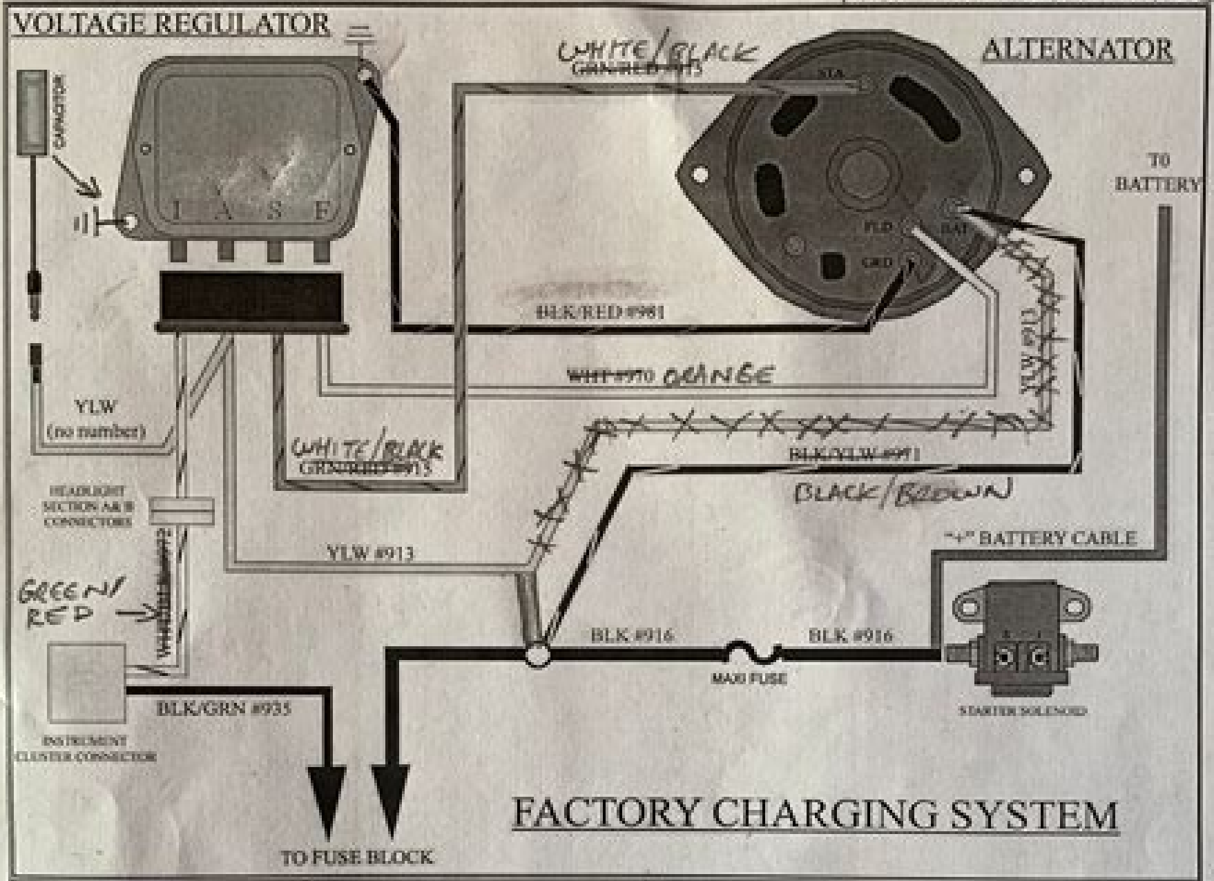
Figure 9 Ford Alternator
