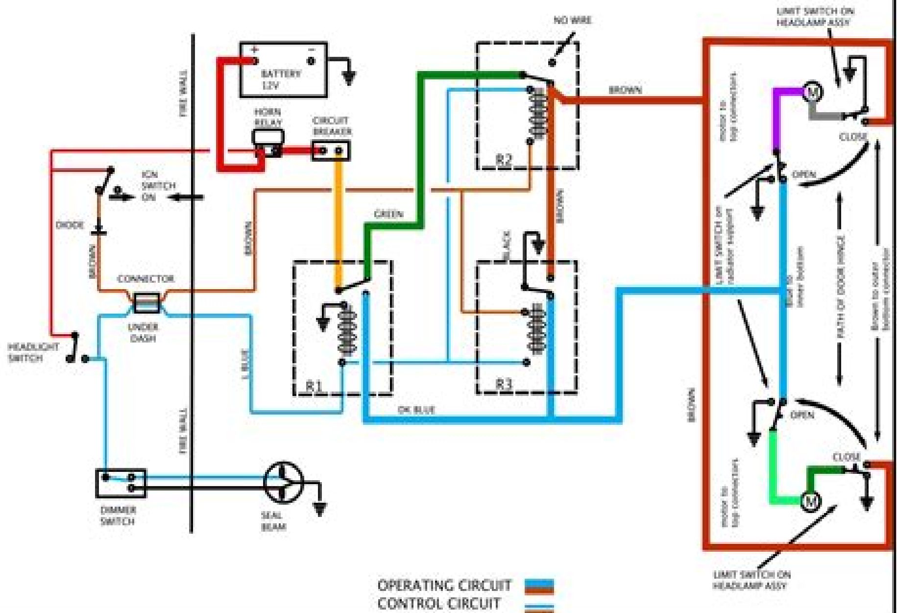
67 CAMARO HEADLAMP DOOR WIRING - LIGHTS OFF, IGN ON, DOORS CLOSED.
