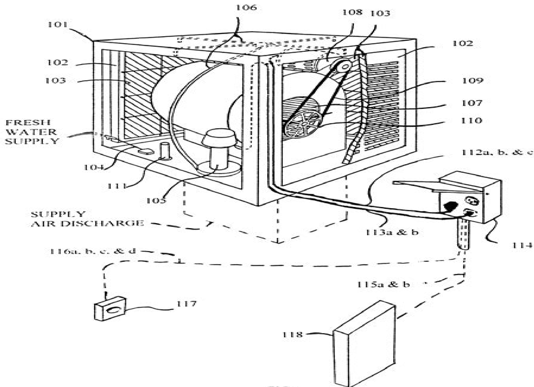
FIG 1 PRIOR ART EVAPORATIVE COOLER AND WIRING
