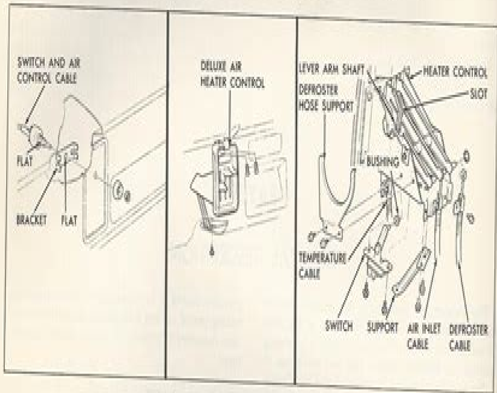
Fig. 2—Heater Controls
