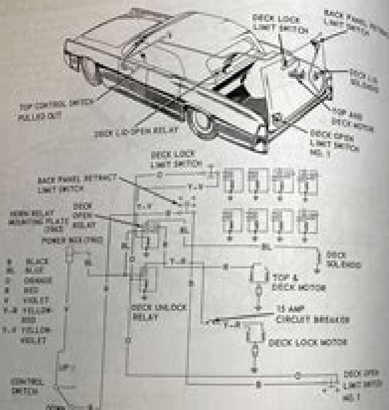
TOP RETRACT CYCLE (Cont.)
