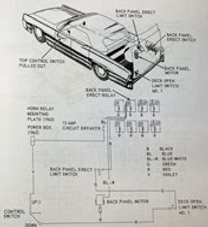
TOP RETRACT CYCLE (Cont.)
