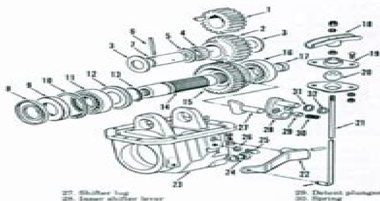
Fig. 14—Exploded view of front-wheel drive transfer gearbox.
