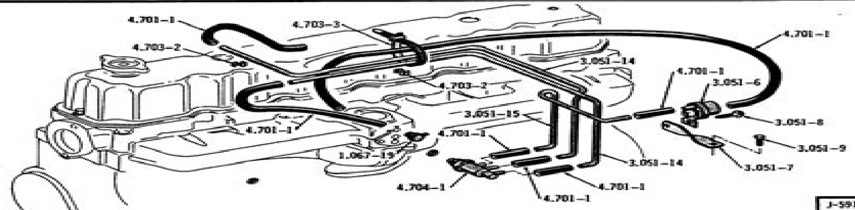
VACUUM ADVANCE MODULATION SYSTEM . . . 80 (SIX-E/ CALIF)
