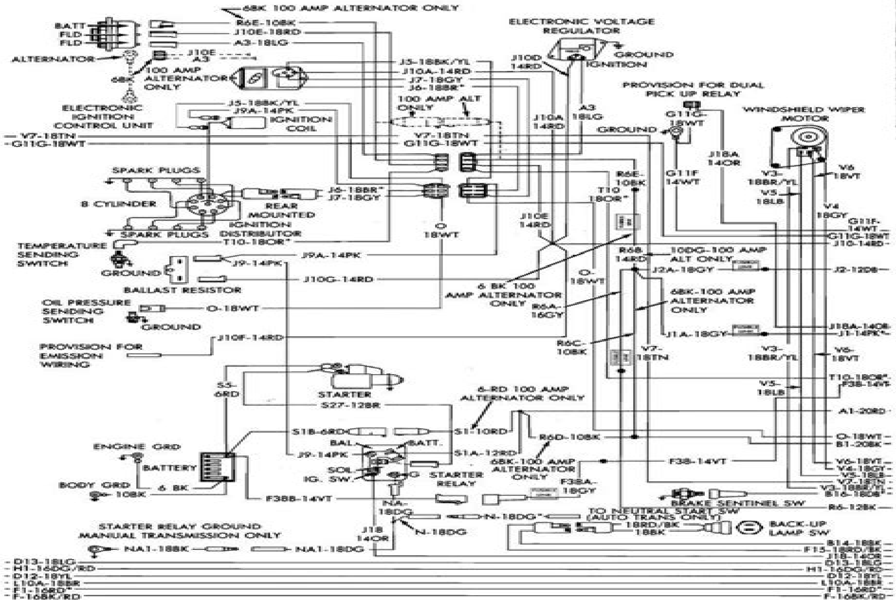
Engine Compartment Wiring Diagrams 8 Cylinder ECU Ignition
