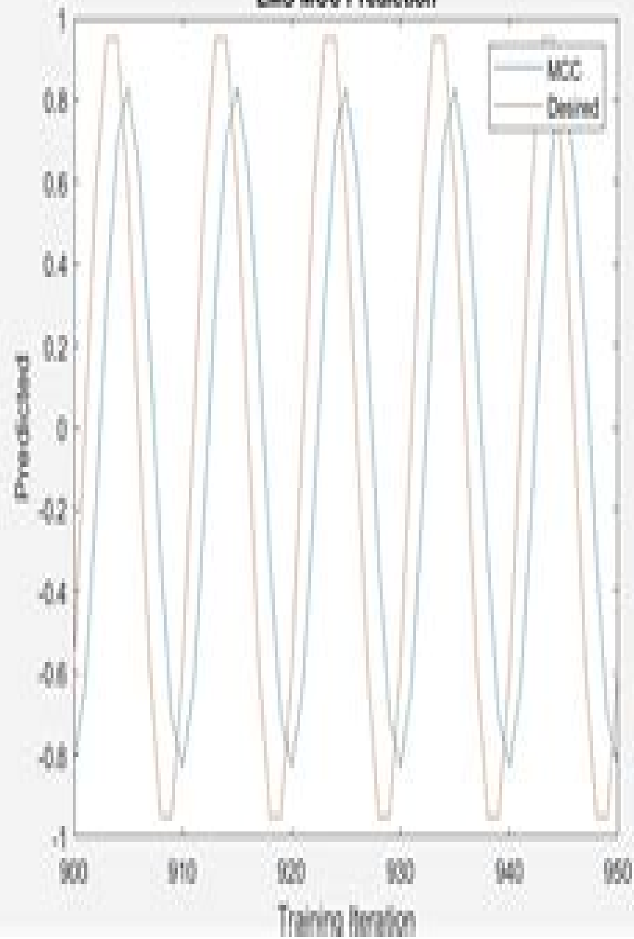
LMS MCC Prediction
