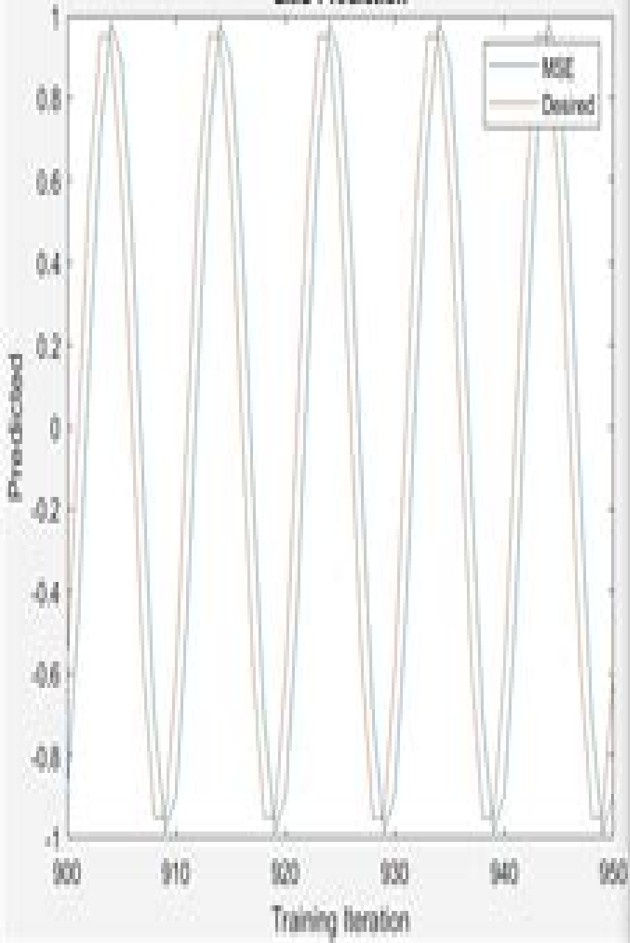
LMS Prediction
