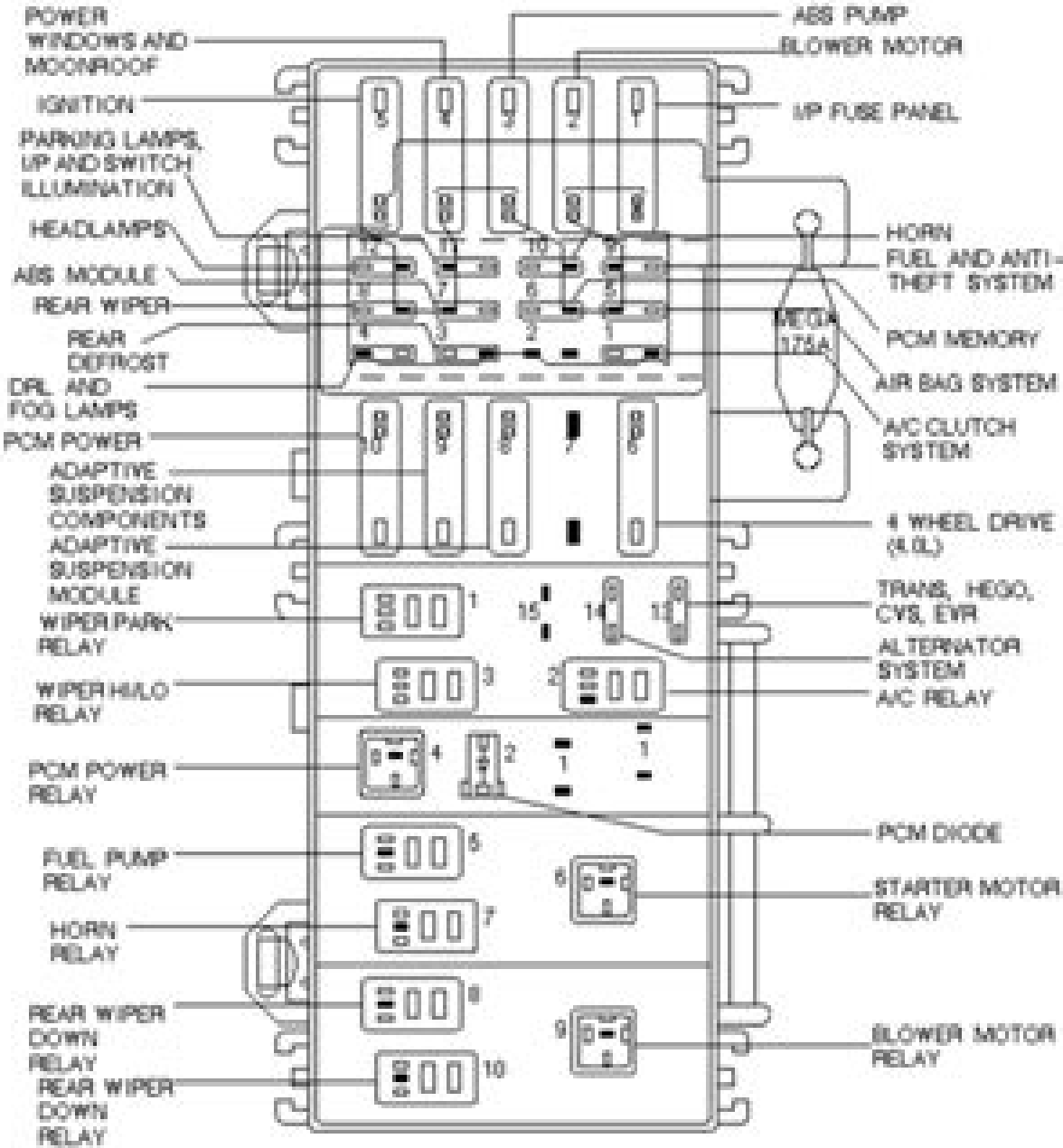
POWER DISTRIBUTION BOX
