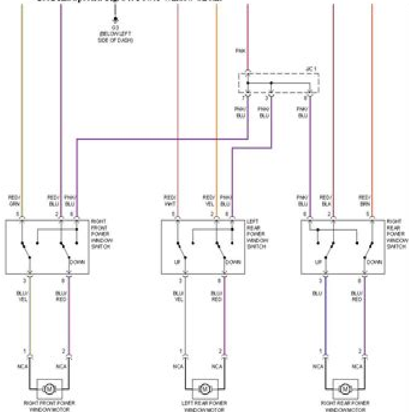
2002 Kia Spectra-Fig. 34: Power Window Circuit
