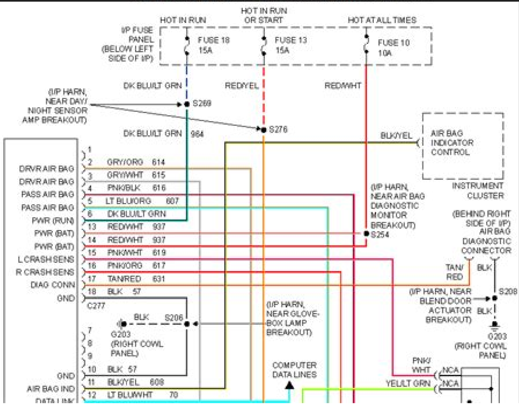
1997 Ford Crown Victoria - Fig. 54: Supplemental Restraint Circuit
