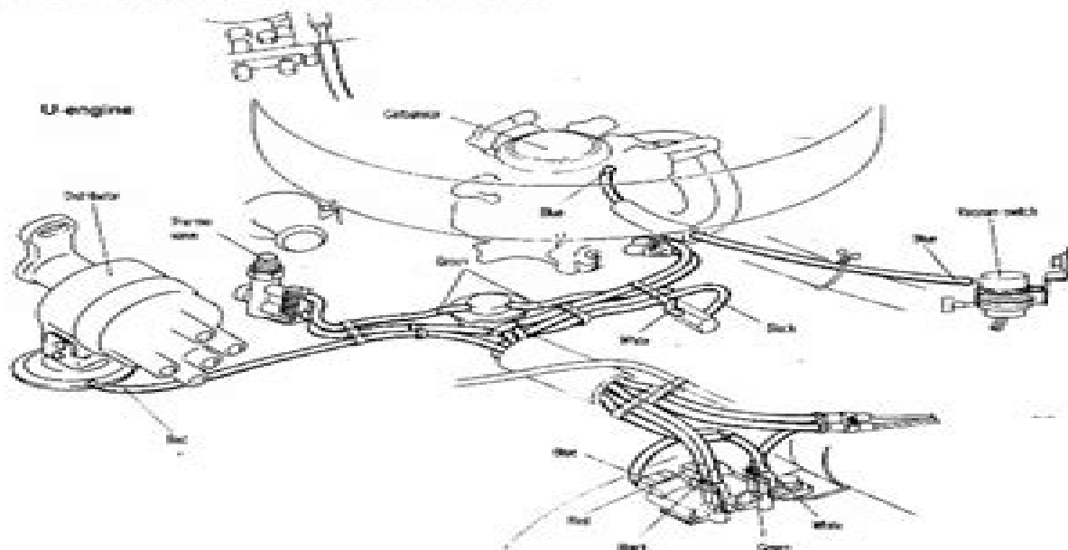
1.3a Vacuum schematic (1985 and 1986 2.5L engine shown, 2.6L engine similar)
