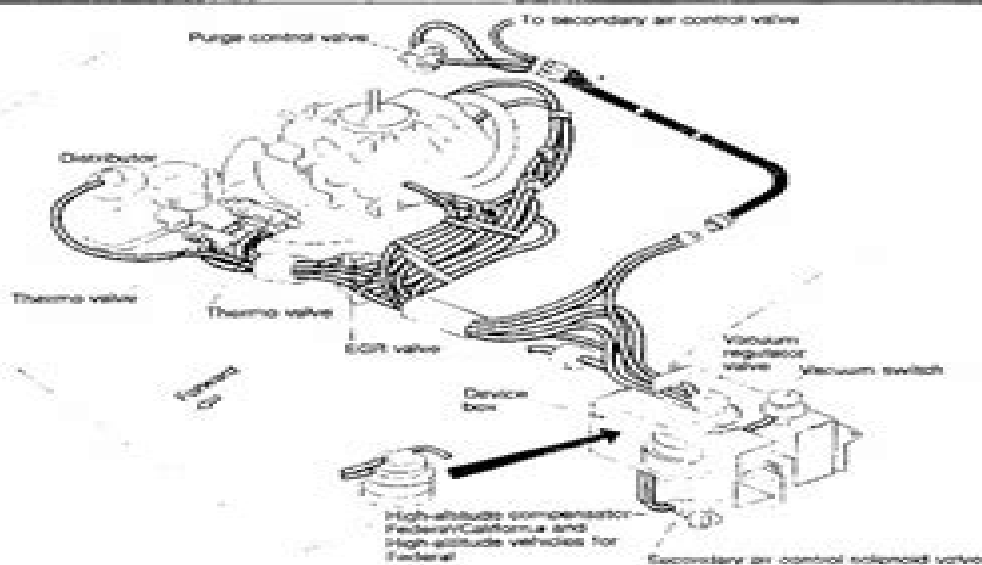
1.3b Vacuum schematic (1987 through 1989, all engines)
