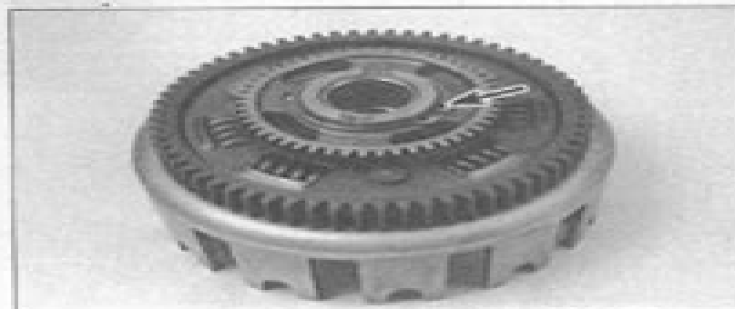
19.11 Remove the snap-ring (arrow) and take off the oil pump drive gear
