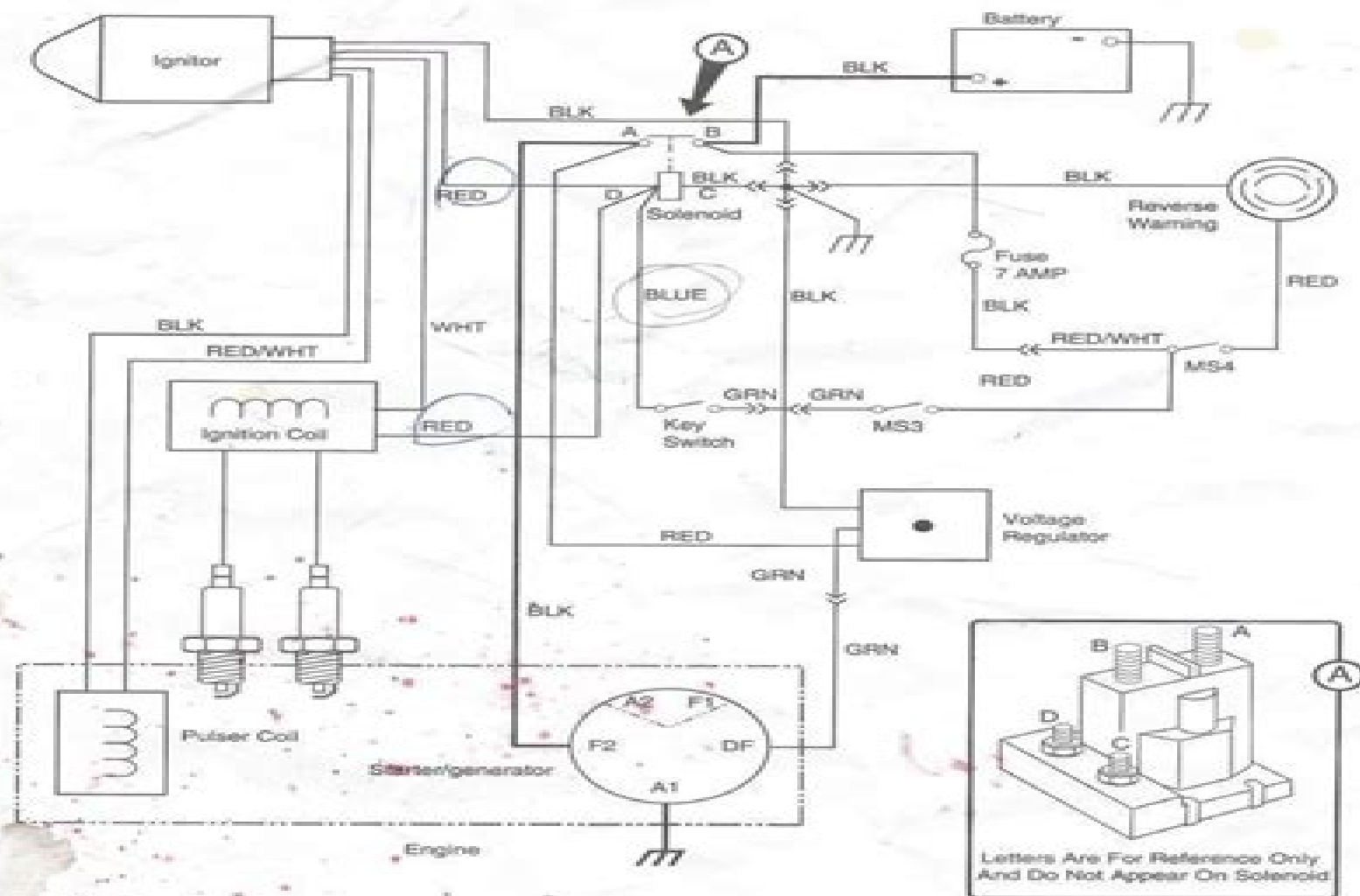
Fig. 1 Electrical System Wiring Diagram
