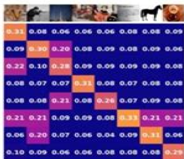
Sigmoid_v1's Cosine Similarity
