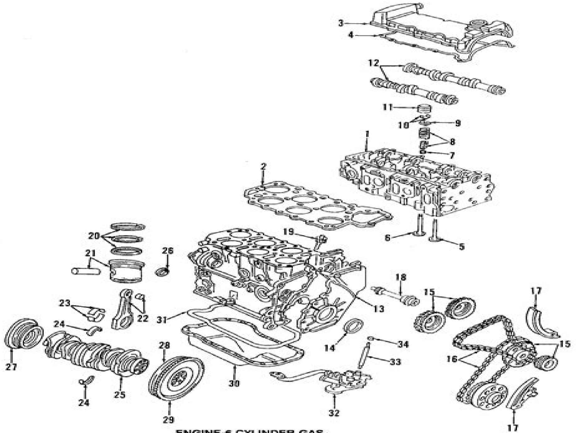
ENGINE-6 CYLINDER GAS
