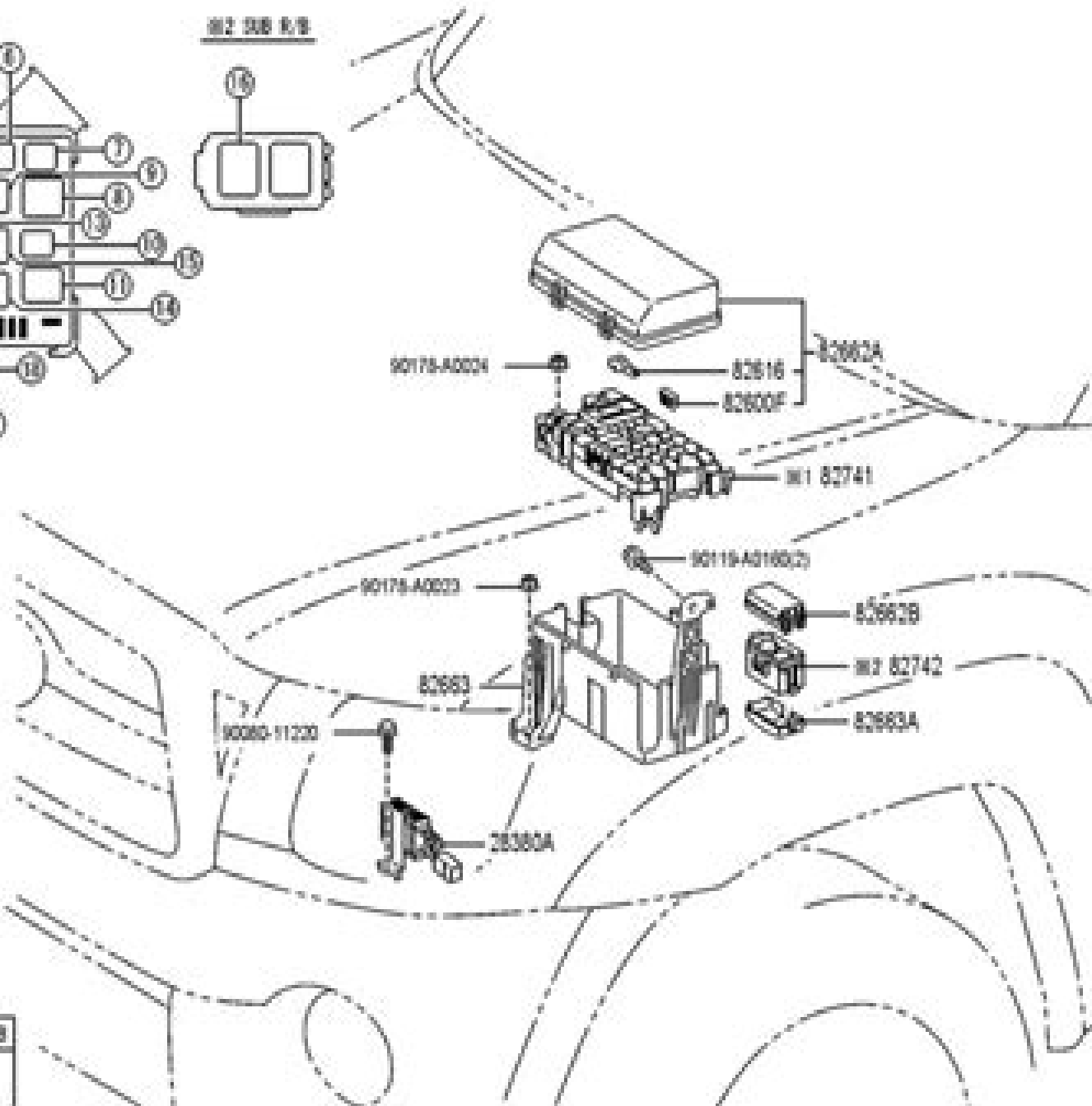
W1 ENGINE ROOM R/R
