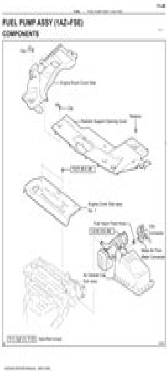
FIG. 10-10-10 FUEL PUMP ASSY (1A2-F10)
