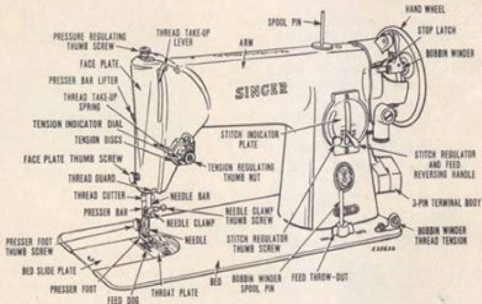
Fig. 2 Names of Principal Parts of Machine 191
