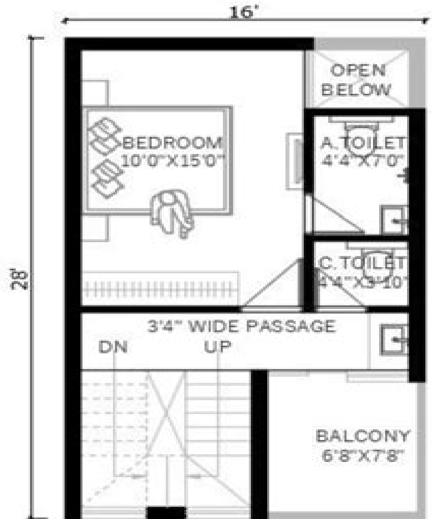
FIRST FLOOR
