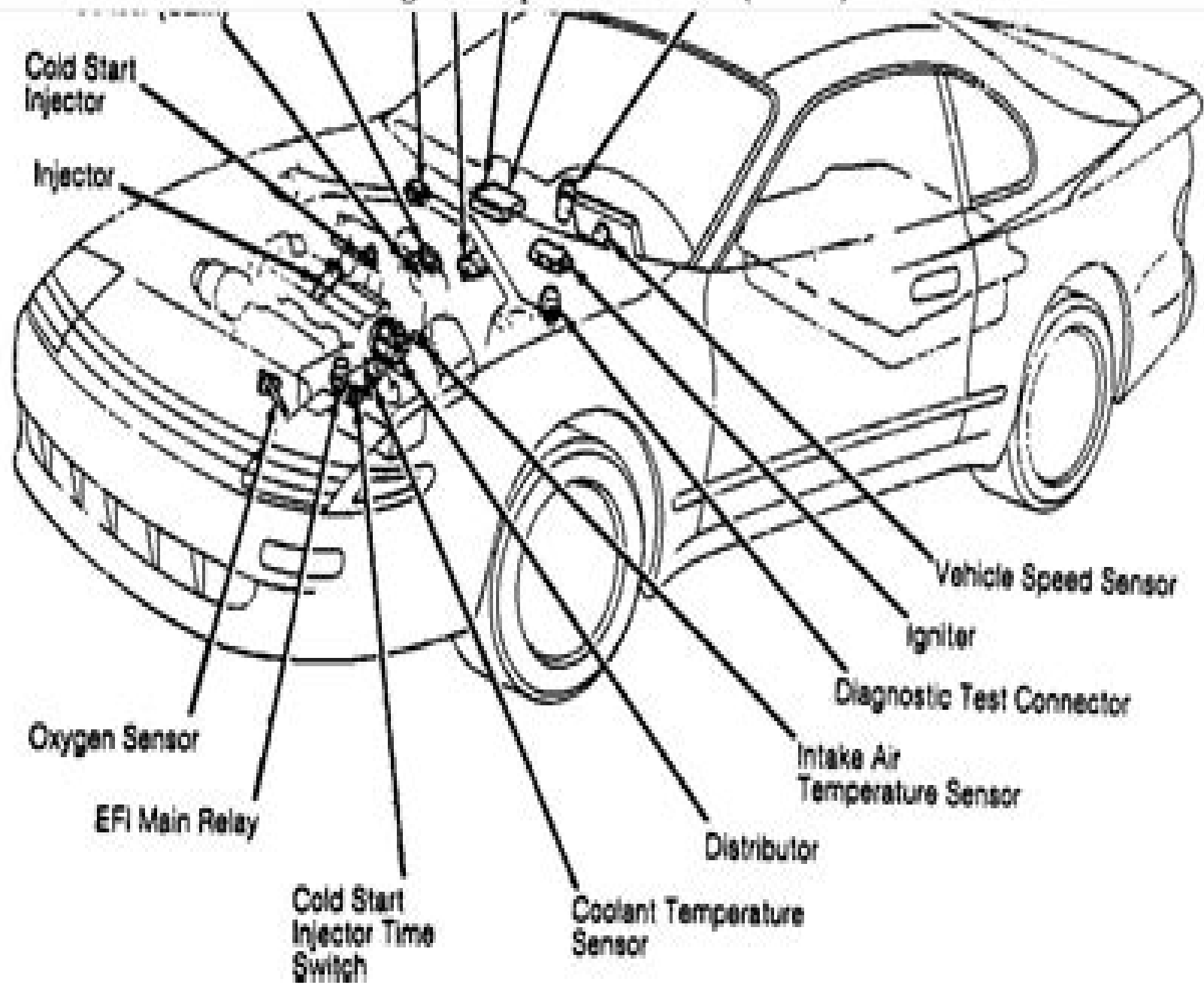
Fig. 5: Component Locations (5 Of 10)
