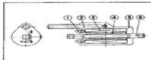
Fig. 155 ① Secondary coil terminal ② Ignition cord ③ Secondary coil ④ Primary coil ⑤ Body ⑥ Core
