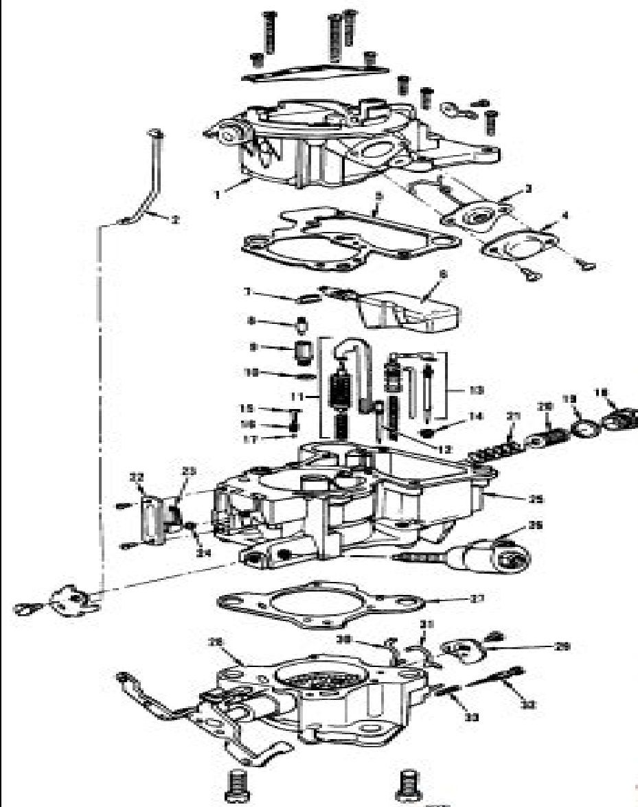
FIGURE 7. CARBURETOR.
