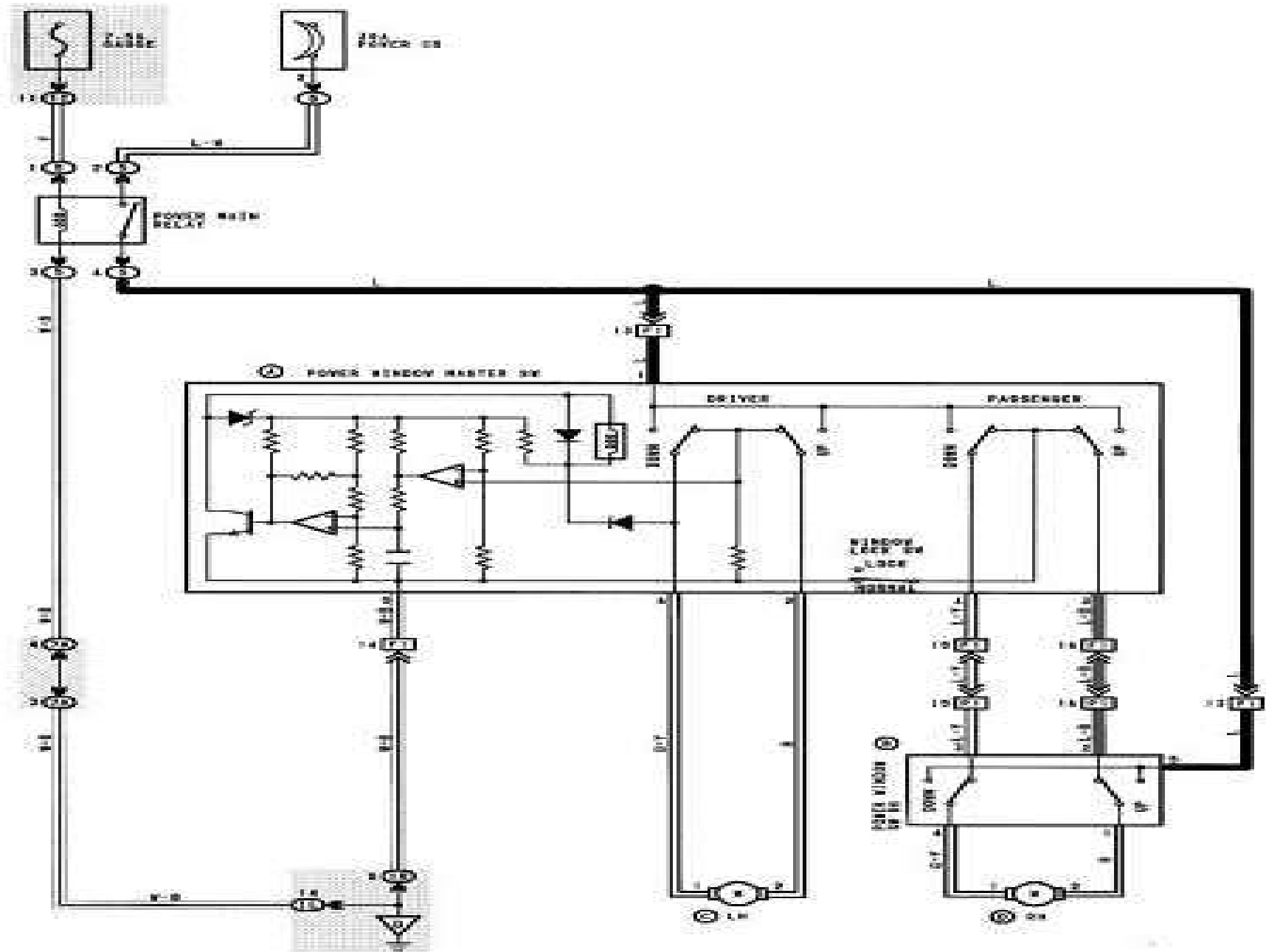
Gambar 1. Rangkaian Power Window (Toyota electrical wiring diagram work book )
