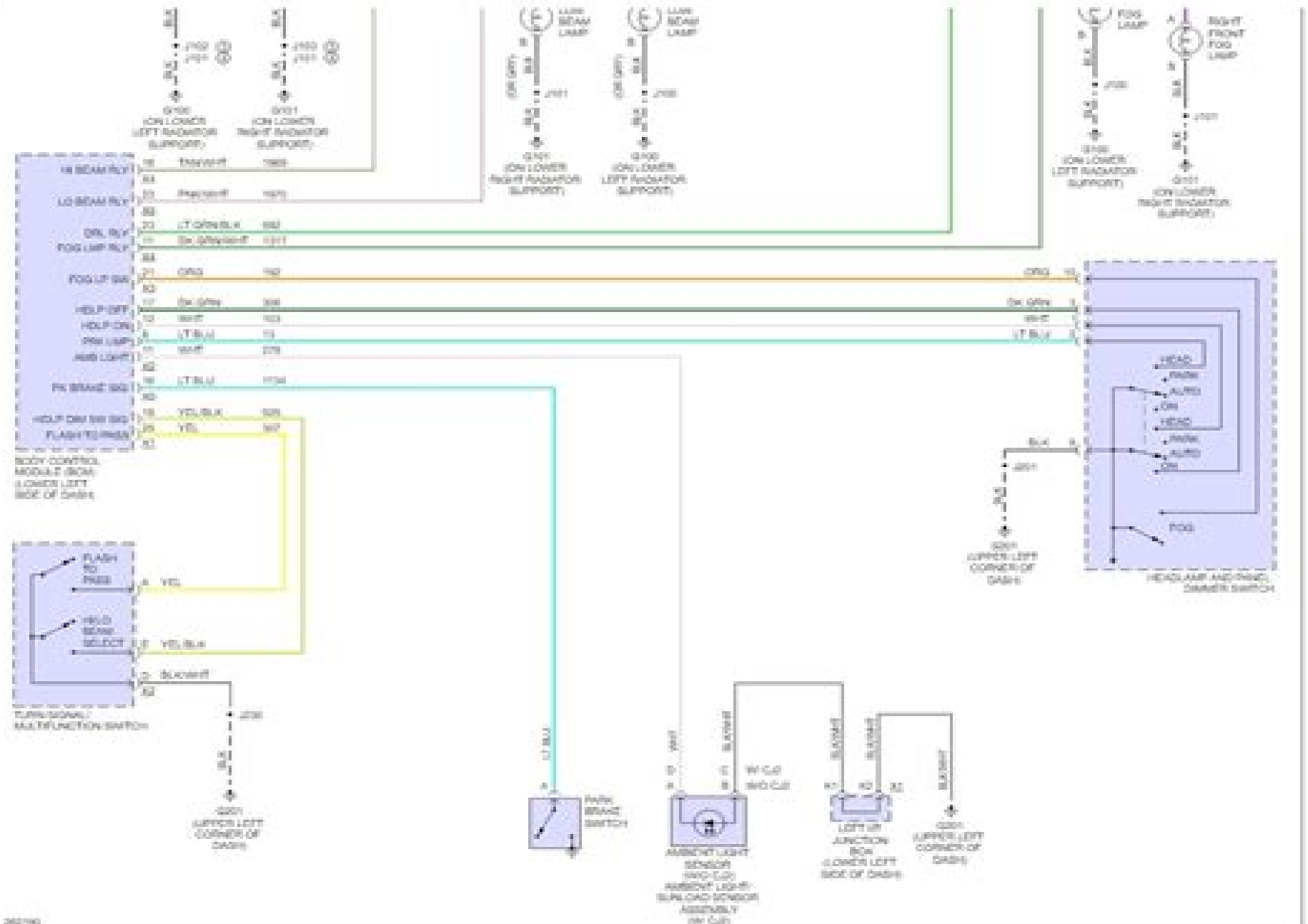
Fig 1: Headlights Circuit
