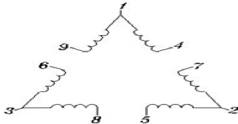
HIGH VOLTAGE "DELTA"
