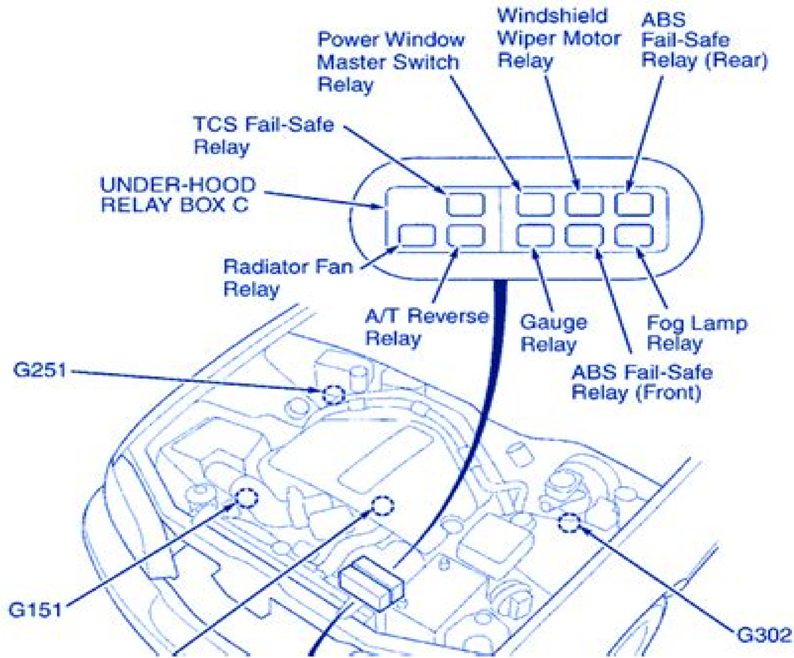
Fig. 7: Engine Compartment
