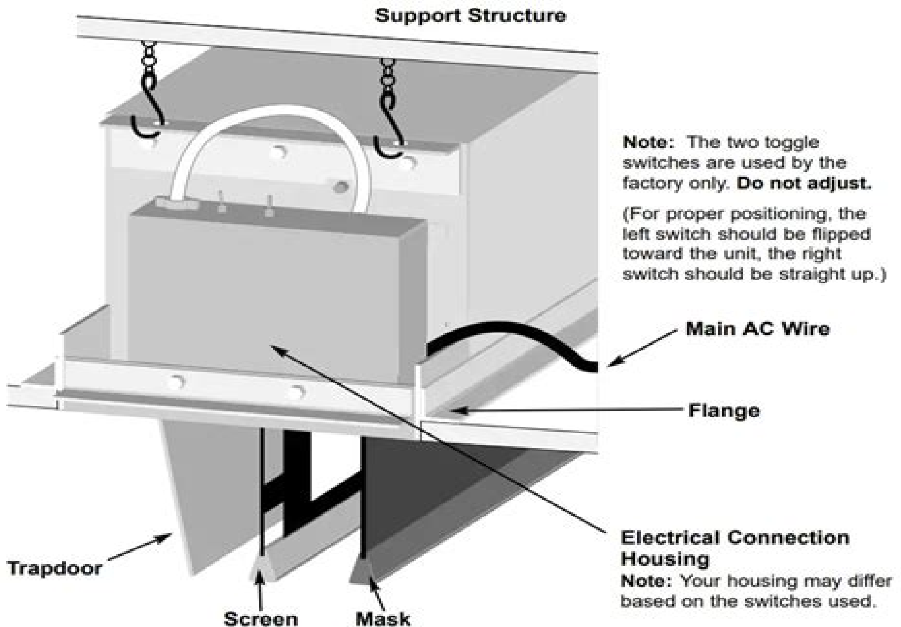
Figure 3: Side view
