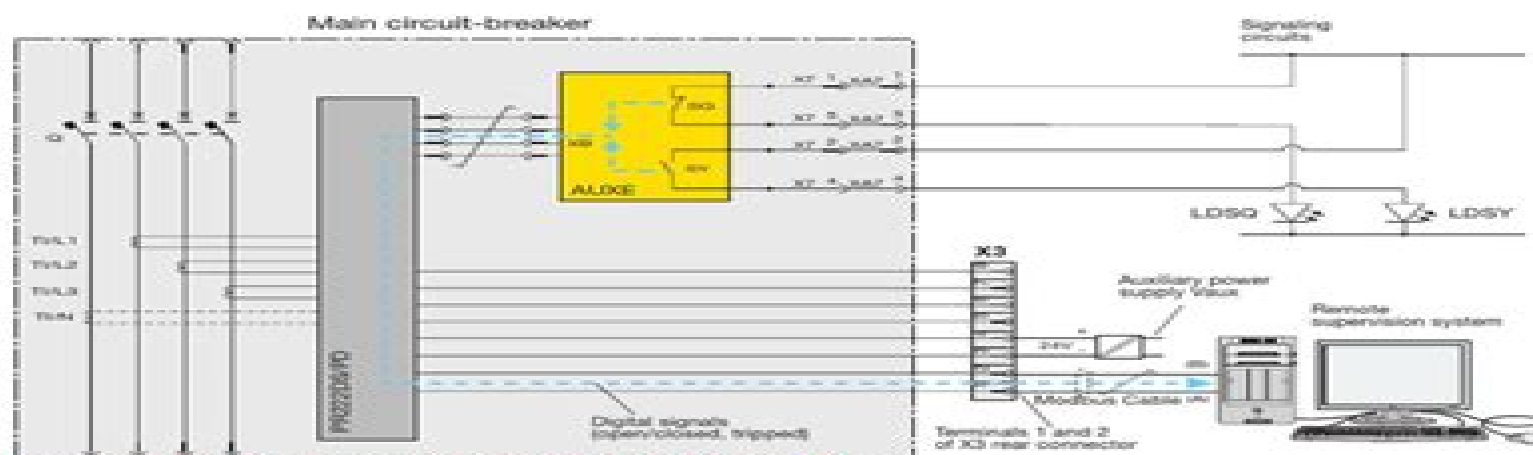
Figure E.2: Wiring diagram of AUX-E contacts connected to PR222DS/PD
