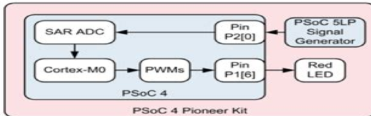
Figure 1. Lab 4 Block Diagram
