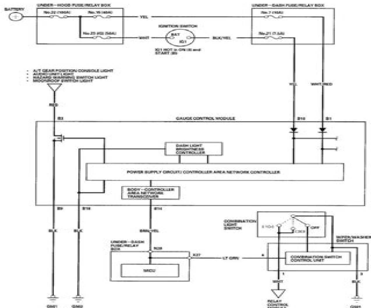
Fig. 1: Dash Lights Brightness Controller Wiring Diagram
