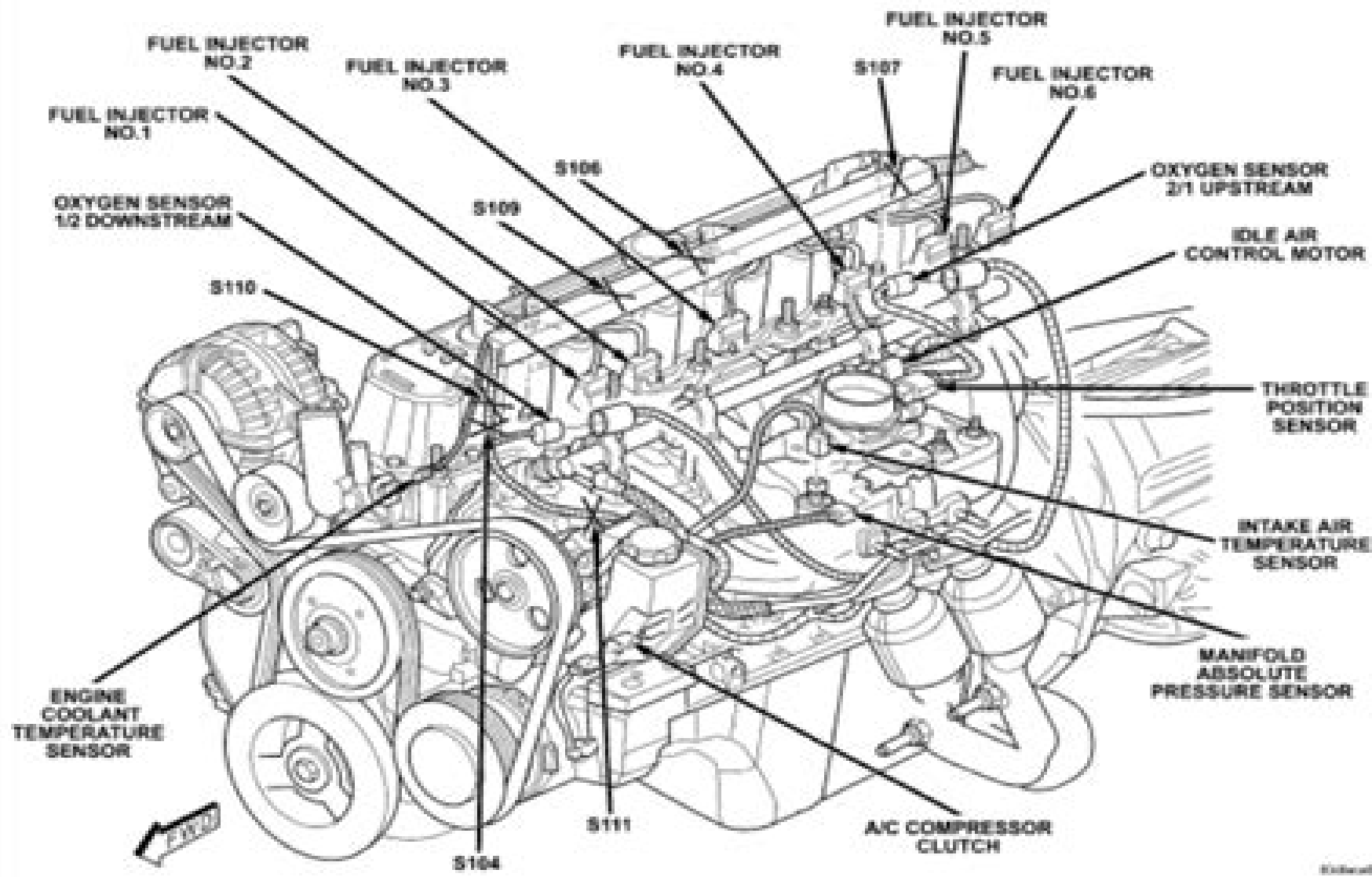
Fig. 14 4.0 LITER ENGINE LEFT SIDE
