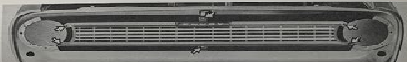
Fig. 3-15 Head lamps removed to show the radiator grille outer attaching points, indicated by arrows.
