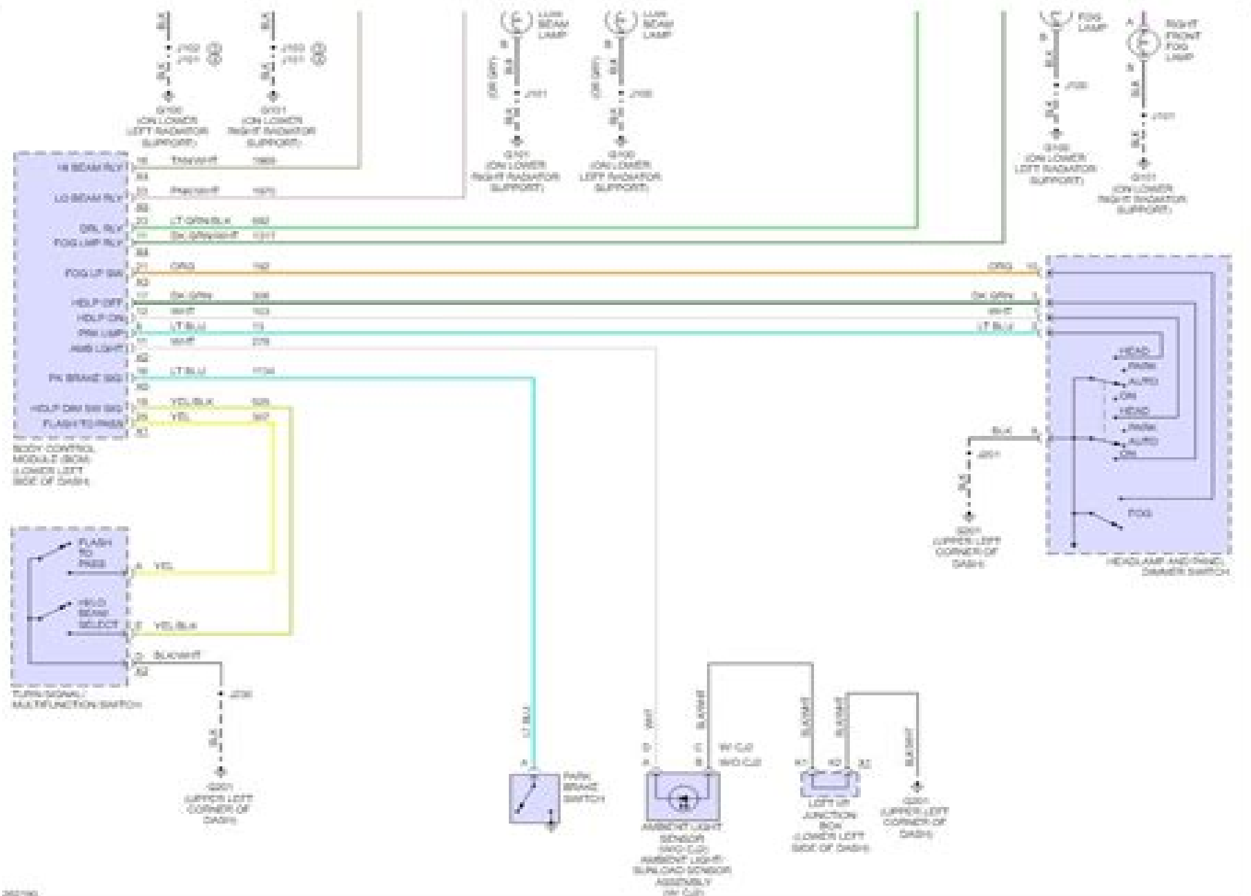
Fig 1: Headlights Circuit
