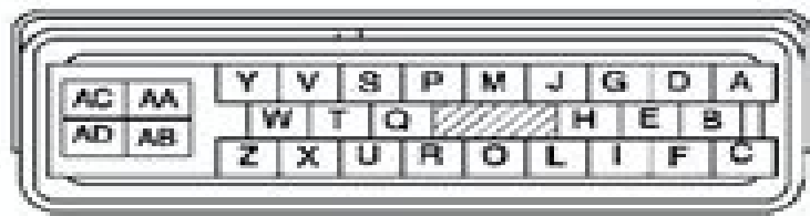
ABS (ABS/TCS) HU/CM HARNESS SIDE CONNECTOR
