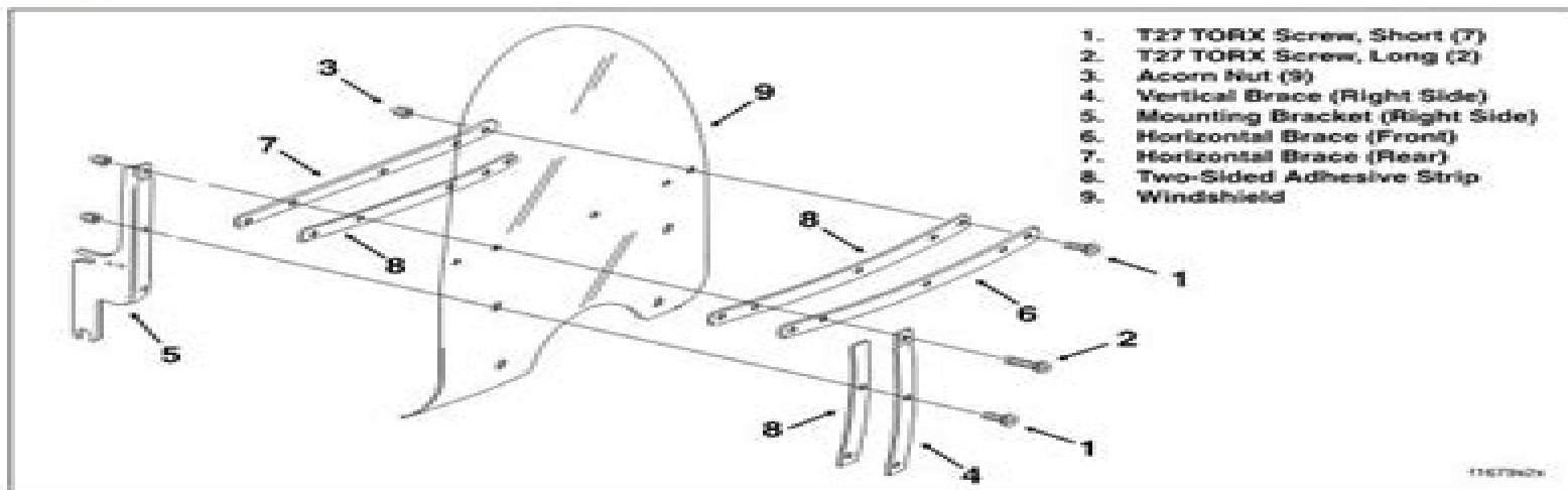
Figure 2-190. Windshield Assembly
