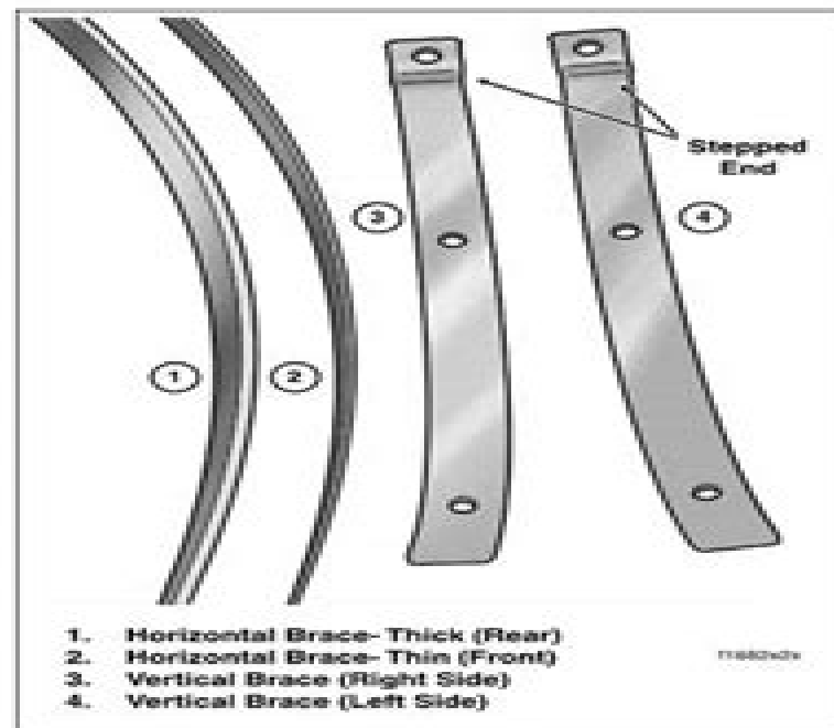
Figure 2-191. Windshield Braces
