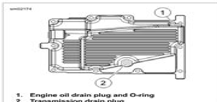
Figure 1-19. Oil Pan
