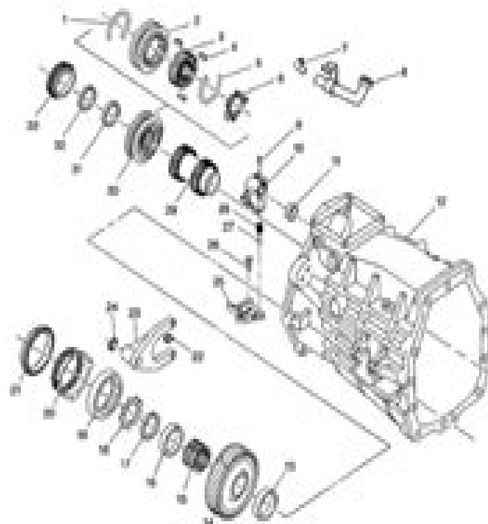
Fig. 5: Transmission Case Component Location (1 of 2) - Y Car Courtesy of GENERAL MOTORS CORP.
