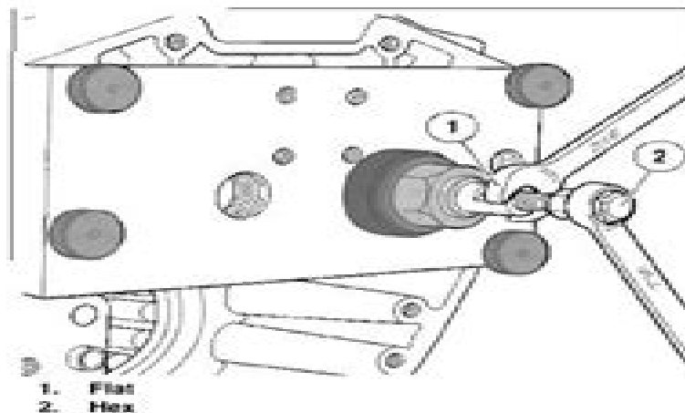
Figure 3-132. Expanding Collet By Turning Hex Clockwise
