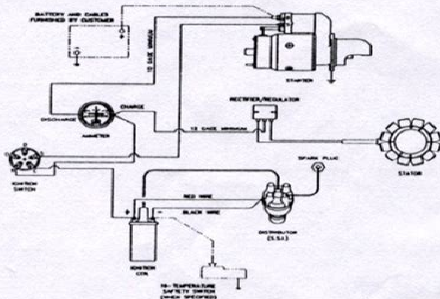
WIRING DIAGRAM, 30 amp Flywheel Alternator with Positive Engage Starter and Solid State Ignition, Models VH4D, VG4D and W4-1770.
