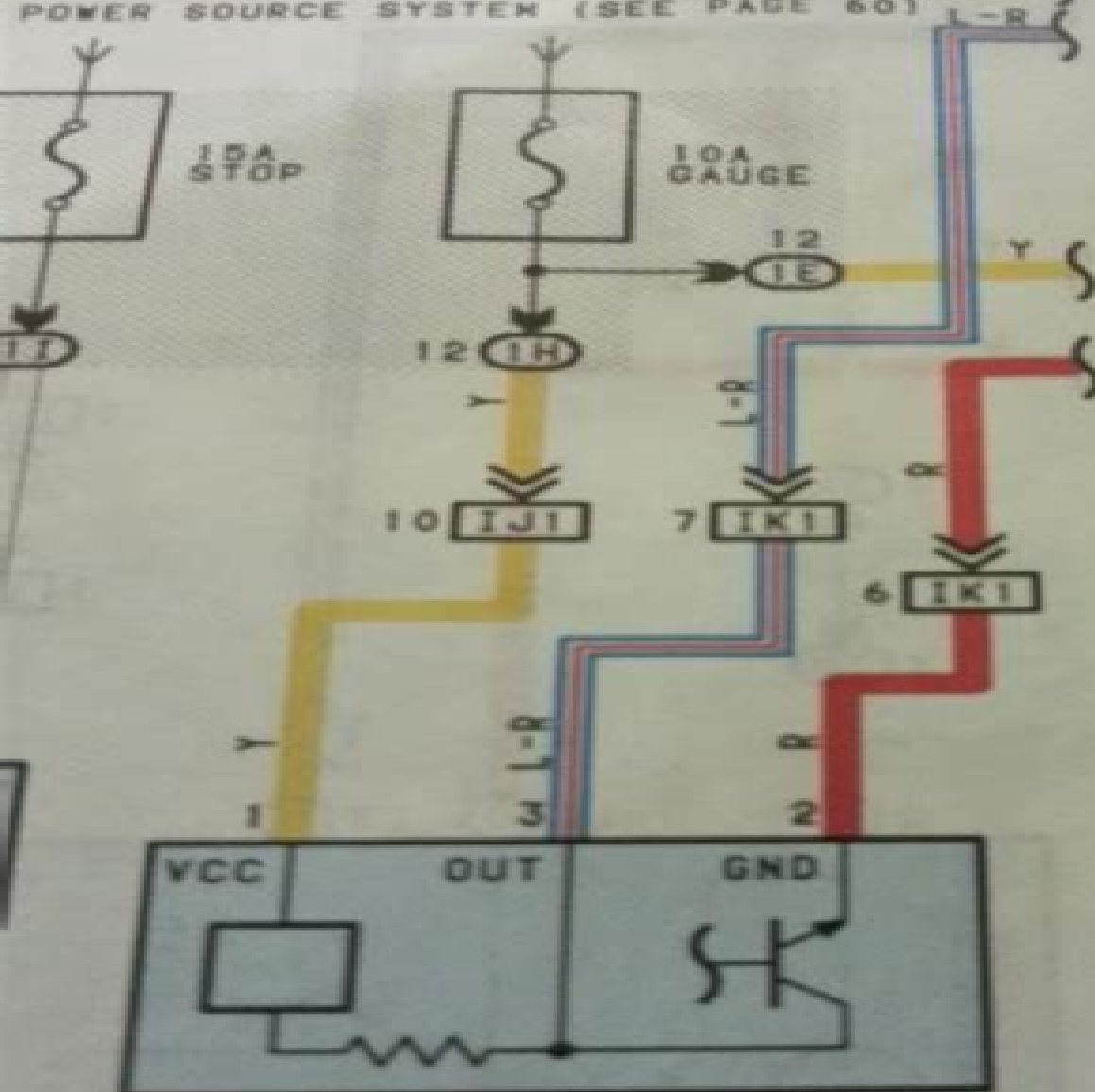
Y 1 VEHICLE SPEED SENSOR NO. 1
