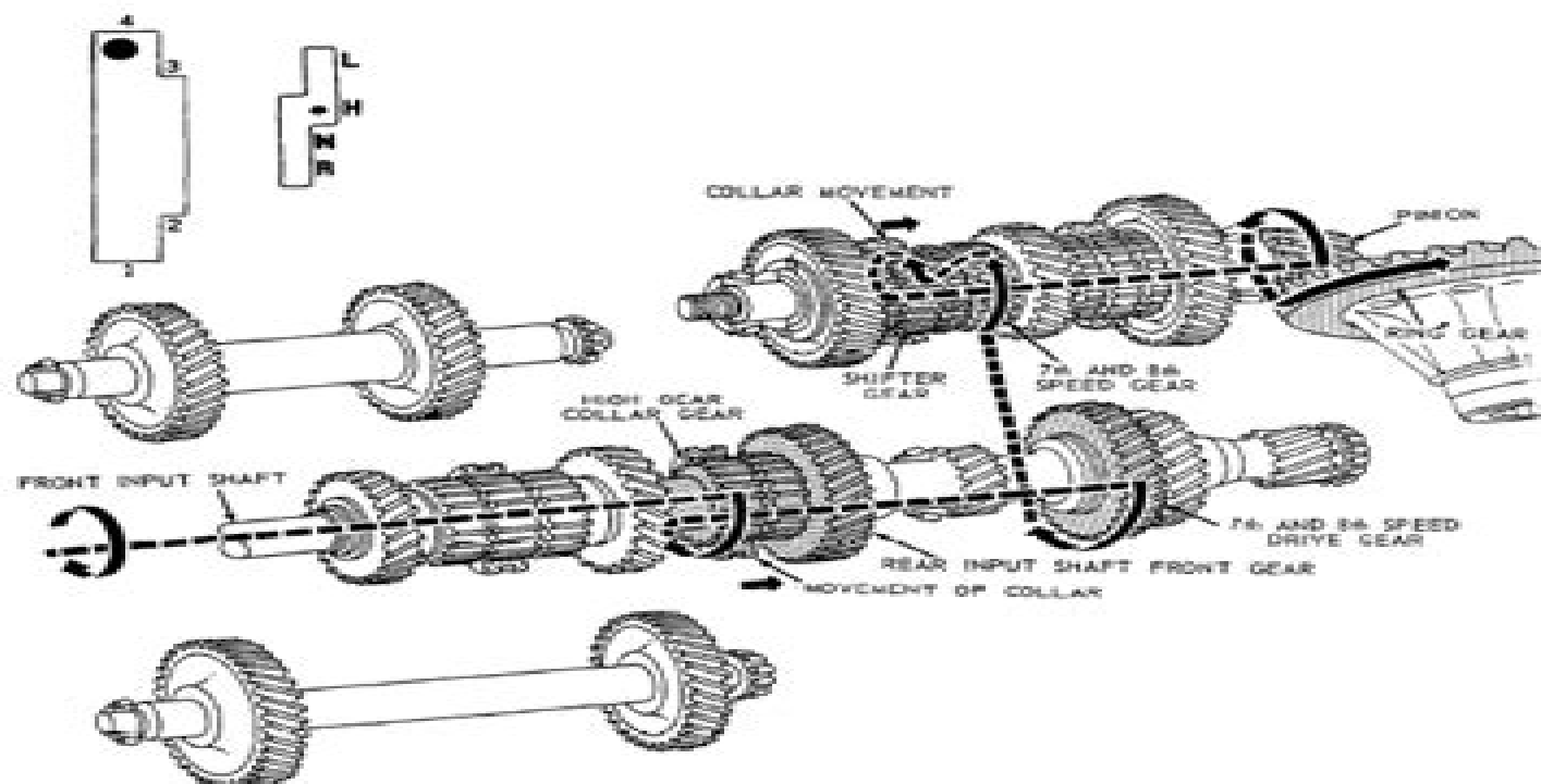
Fig. 120-5-9—Transmission Fourth Shift Station — High Gear
