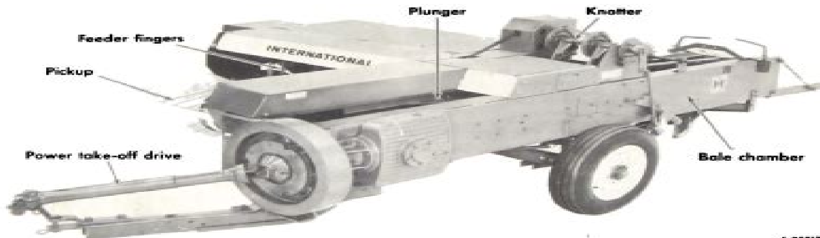
Illust. 2 420 Baler.
