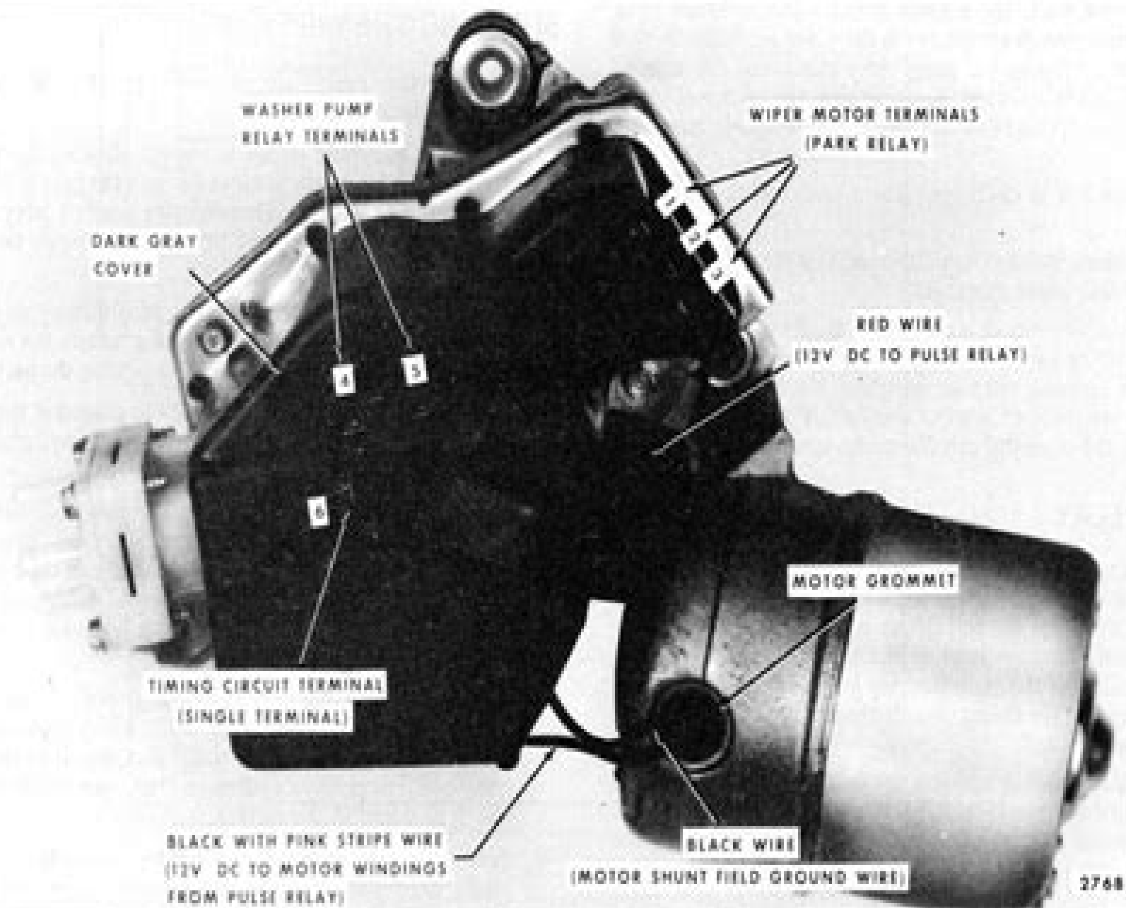
Fig. 2-26-Multiplex Pulse Wiper Motor and Pump Assembly
