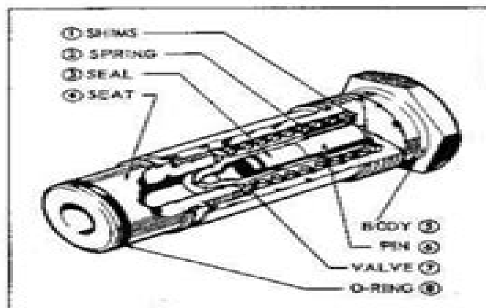
Figure 17 Hydraulic Pressure Relief Valve
