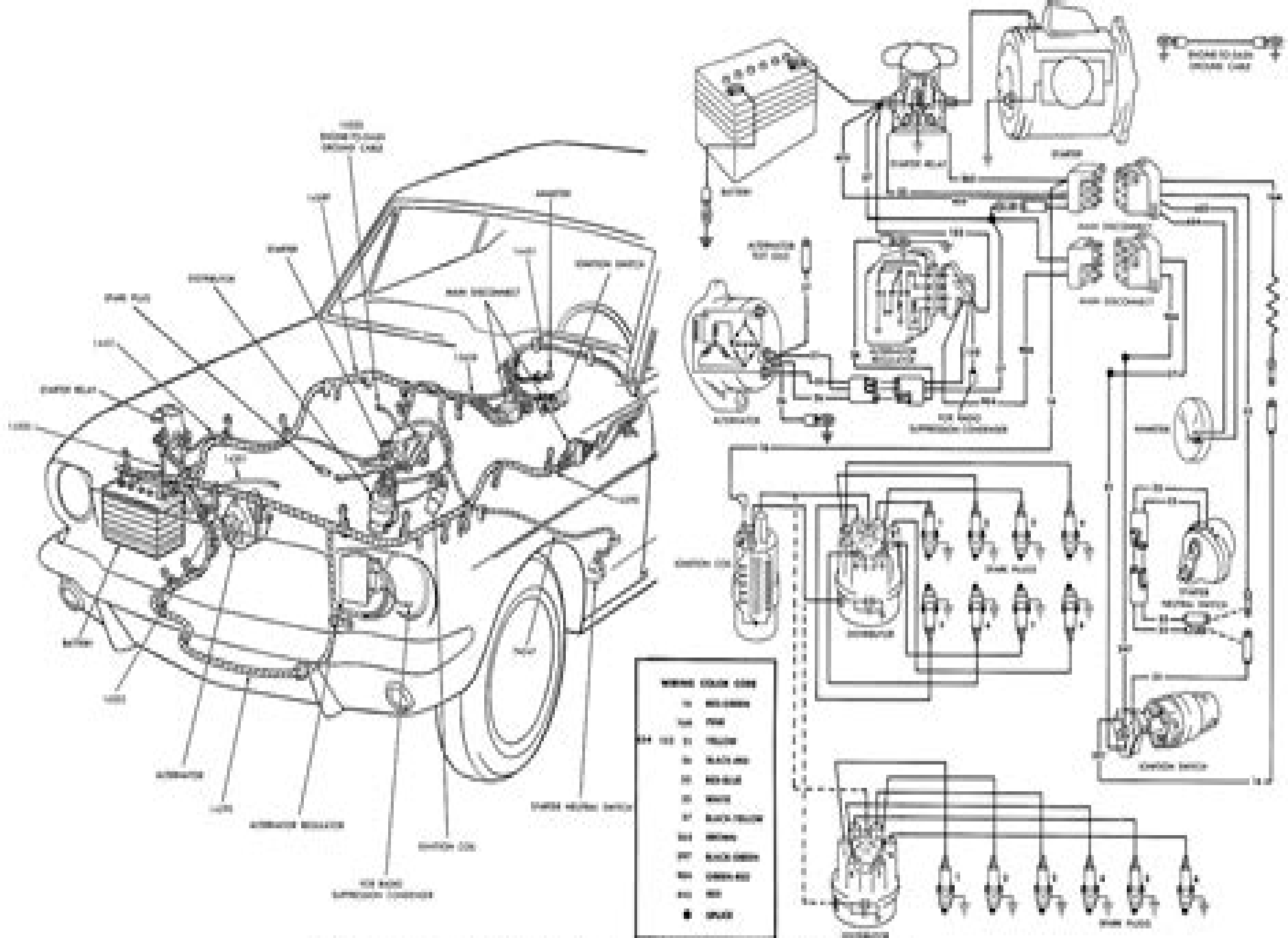
1966 MUSTANG IGNITION, STARTING AND CHARGING
