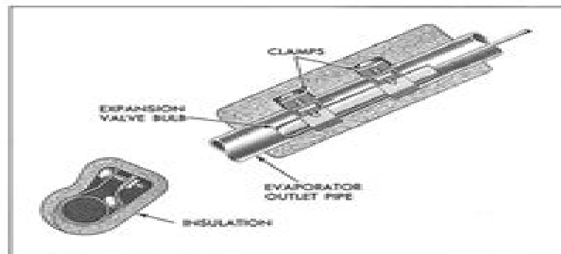
Fig. 2-8 Expansion Valve Bulb at Evaporator Outlet Pipe
