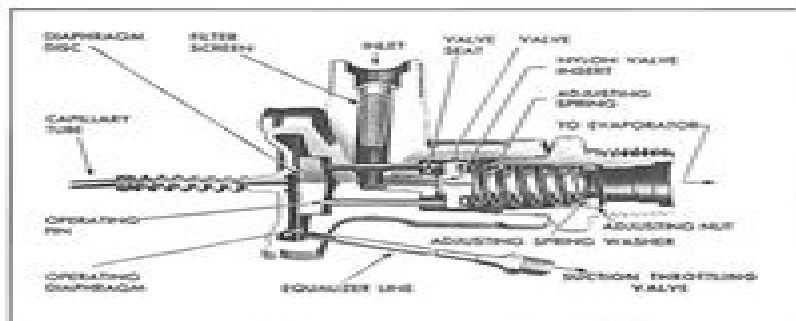
Fig. 2-7 Cross Section - Expansion Valve
