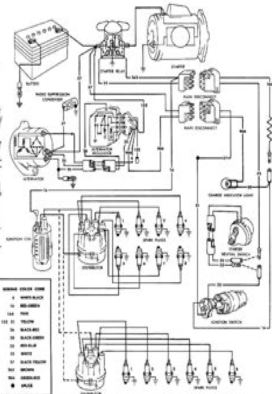
1965 MUSTANG IGNITION, STARTING AND CHARGING
