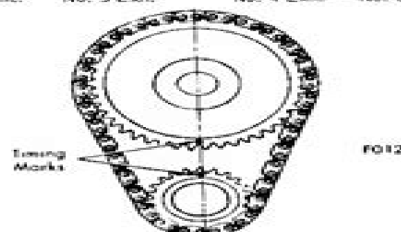
170", 200", 250" VALVE TIMING MARKS
